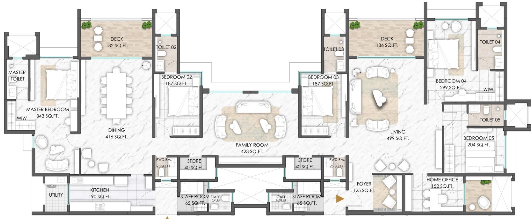
Tower 5 Jodi Unit Plan- Flat 01+02
